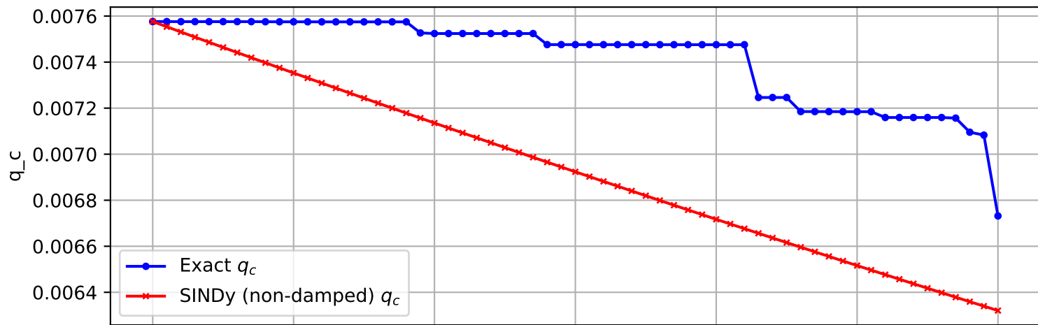
Trajectory 506 (non-damped)
