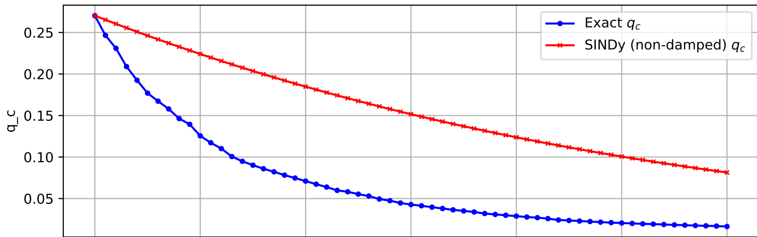
Trajectory 519 (non-damped)
