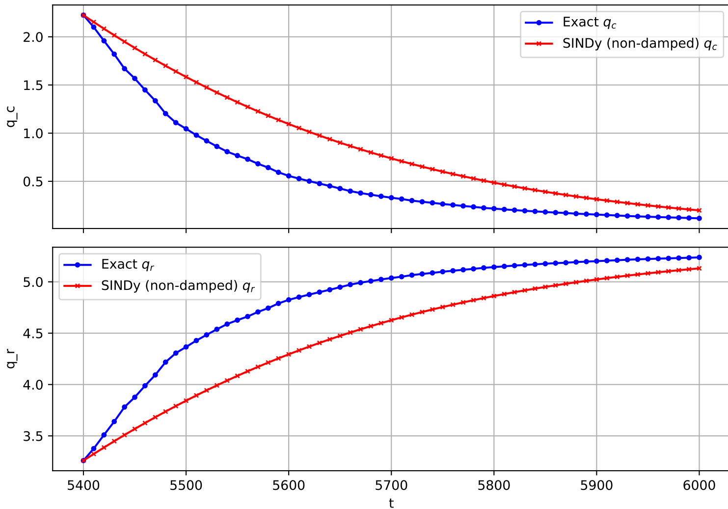
Trajectory 520 (non-damped)
