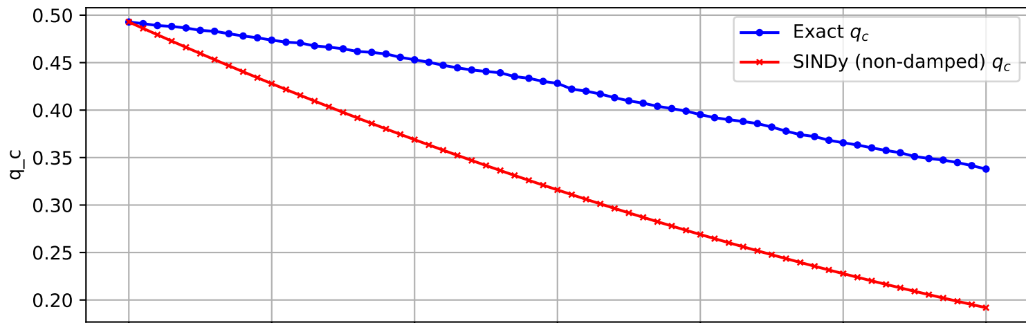
Trajectory 530 (non-damped)
