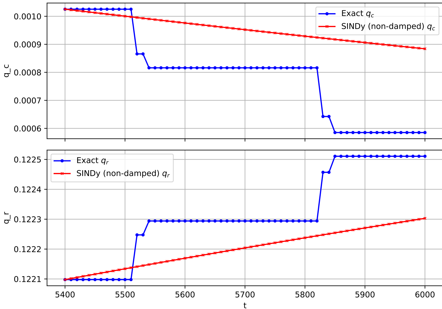
Trajectory 531 (non-damped)
