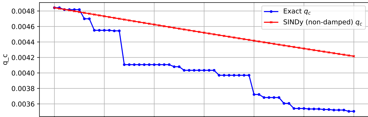
Trajectory 537 (non-damped)
