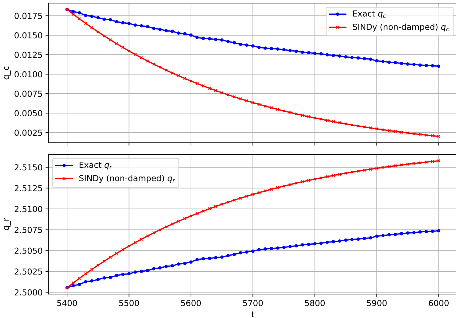
Trajectory 540 (non-damped)
