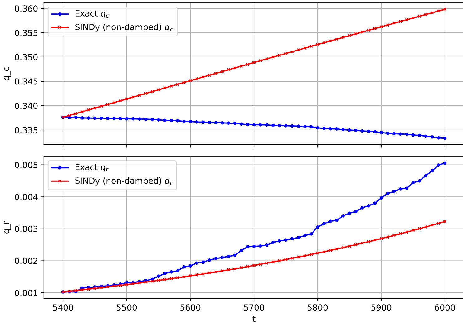
Trajectory 552 (non-damped)
