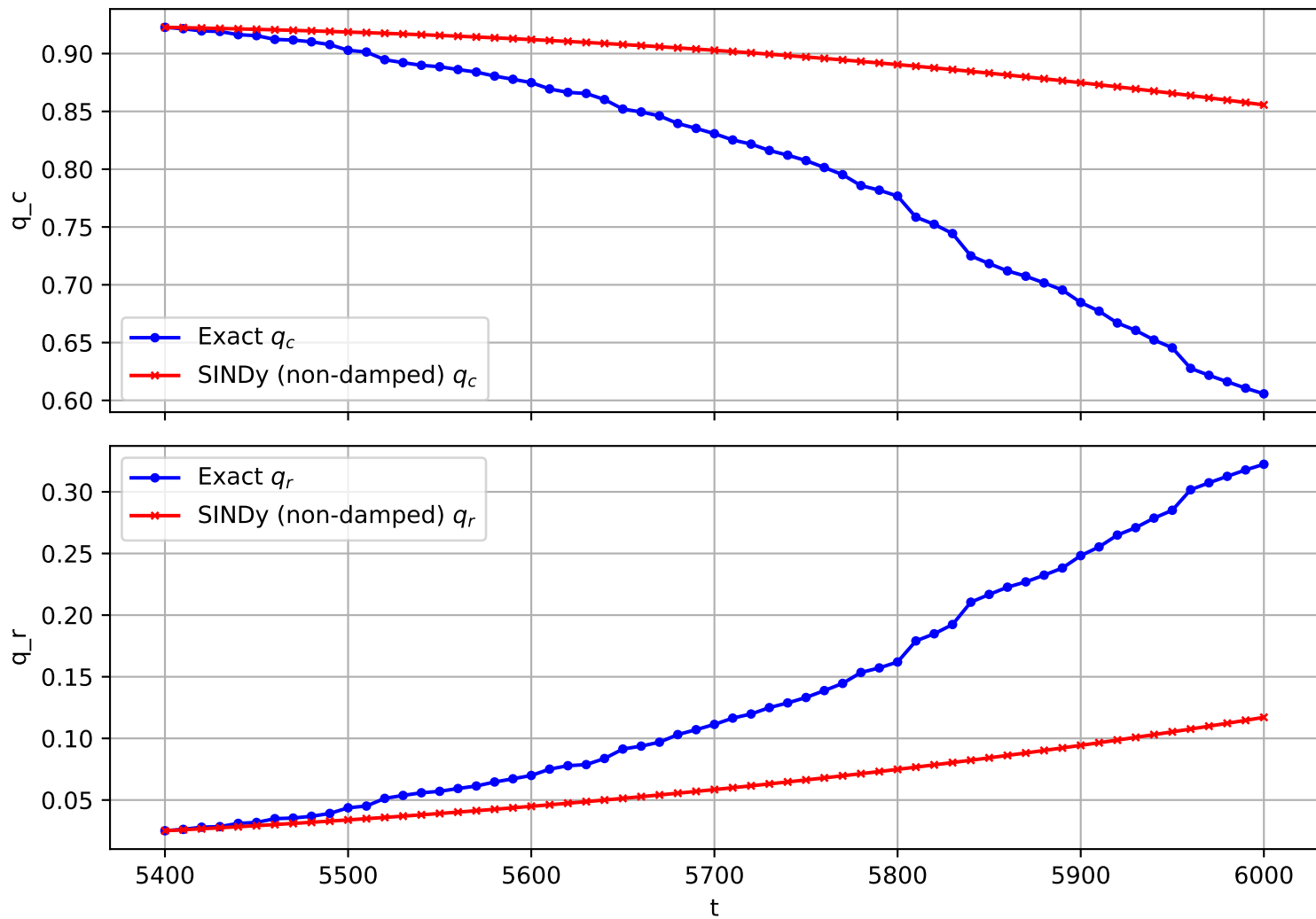
Trajectory 556 (non-damped)
