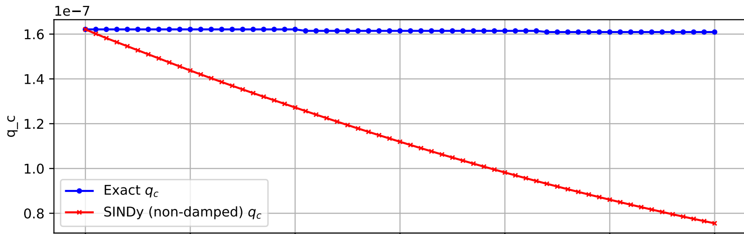
Trajectory 562 (non-damped)
