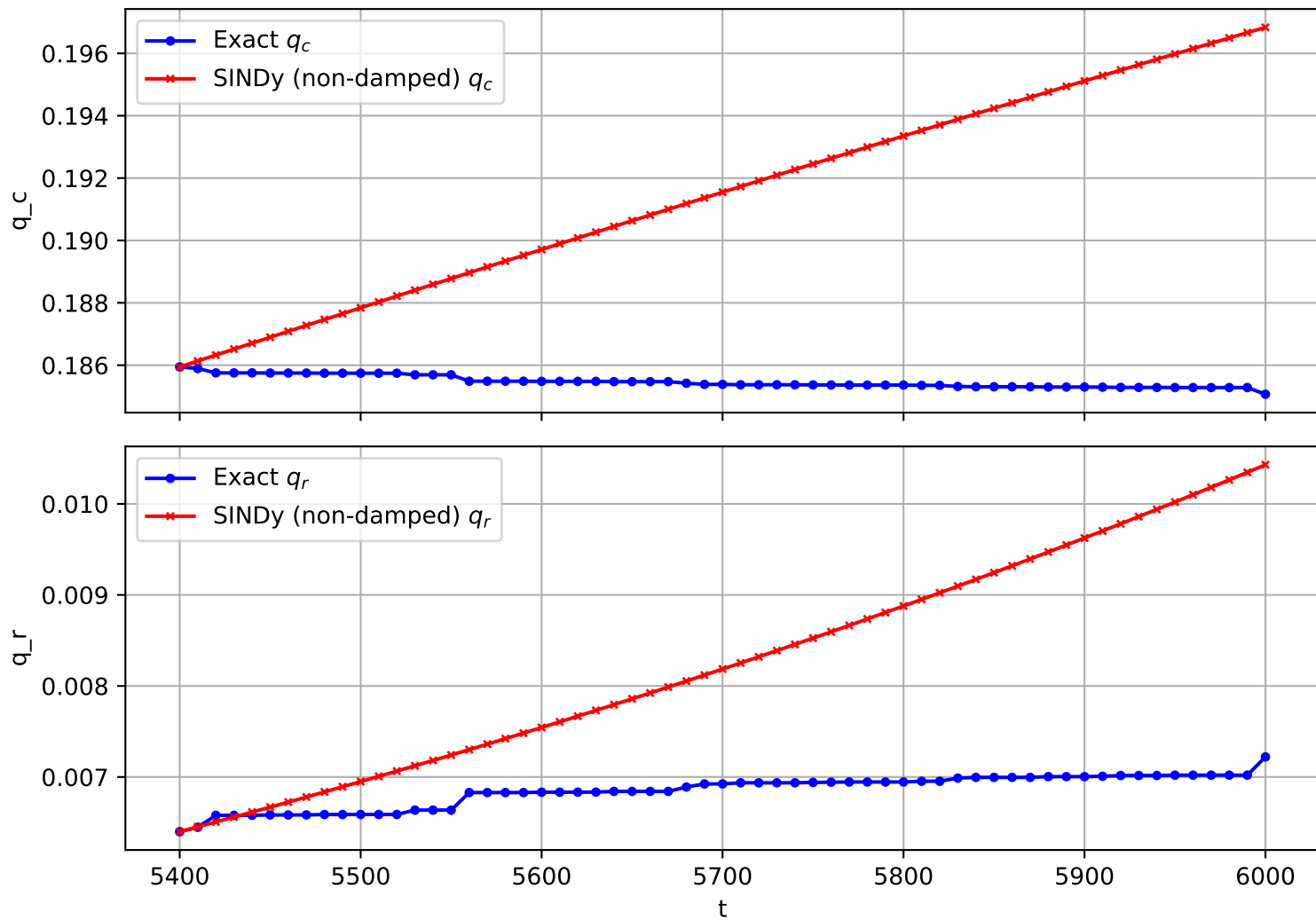
Trajectory 57 (non-damped)
