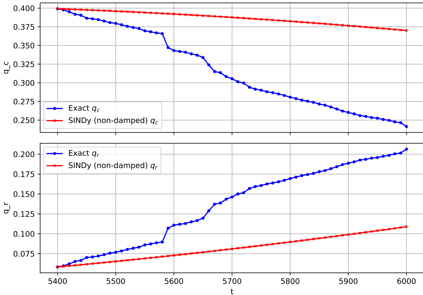
Trajectory 576 (non-damped)
