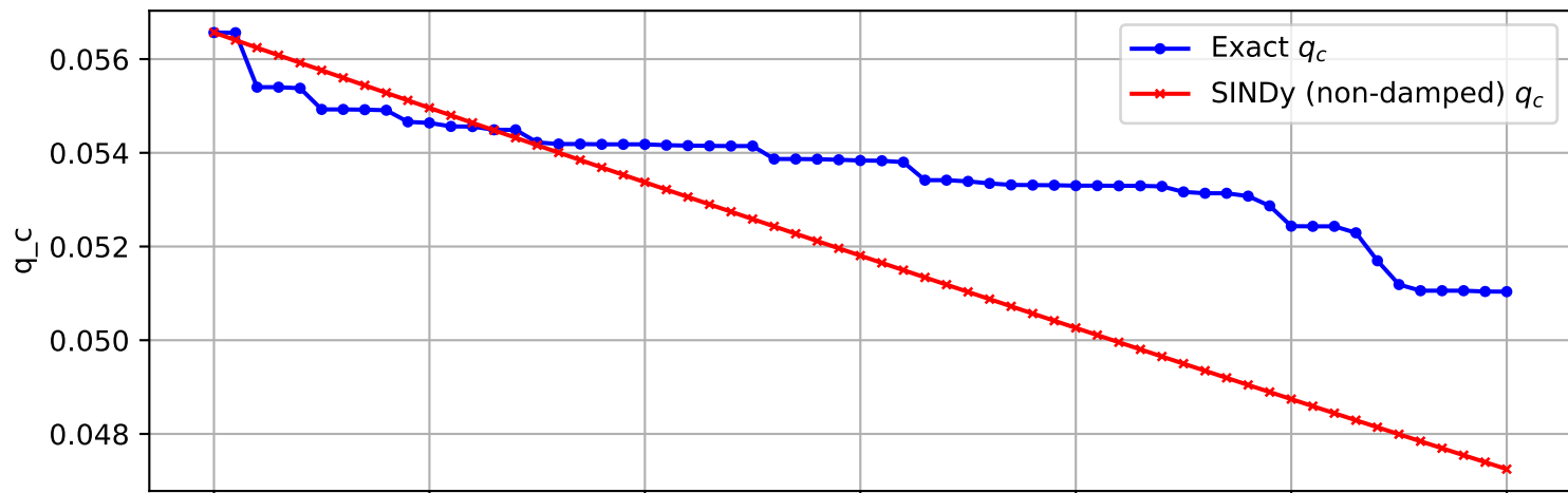
Trajectory 578 (non-damped)
