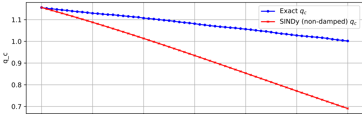
Trajectory 584 (non-damped)
