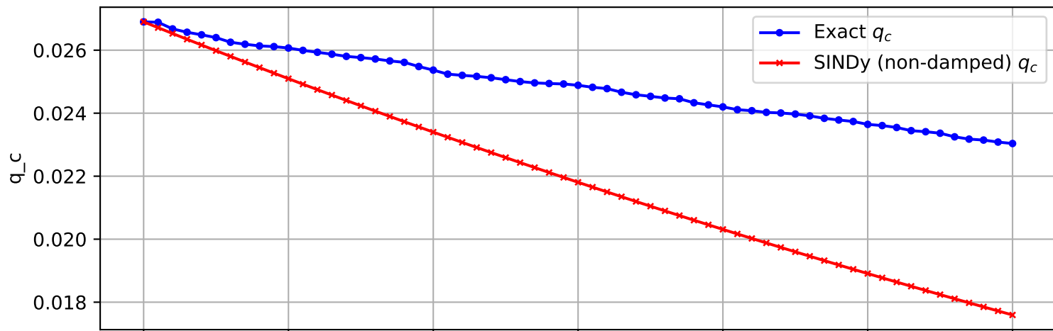
Trajectory 585 (non-damped)
