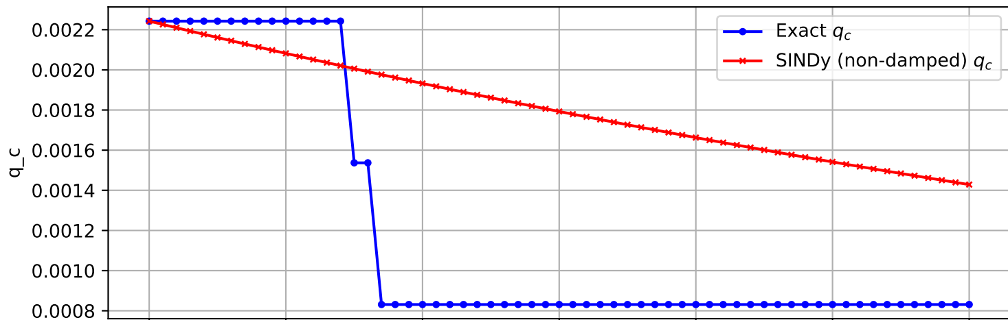
Trajectory 593 (non-damped)
