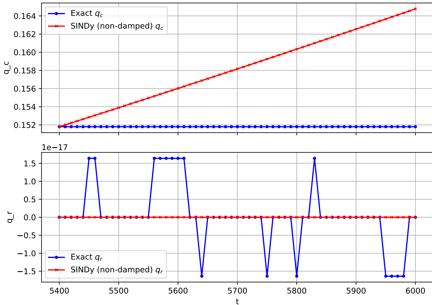
Trajectory 6 (non-damped)
