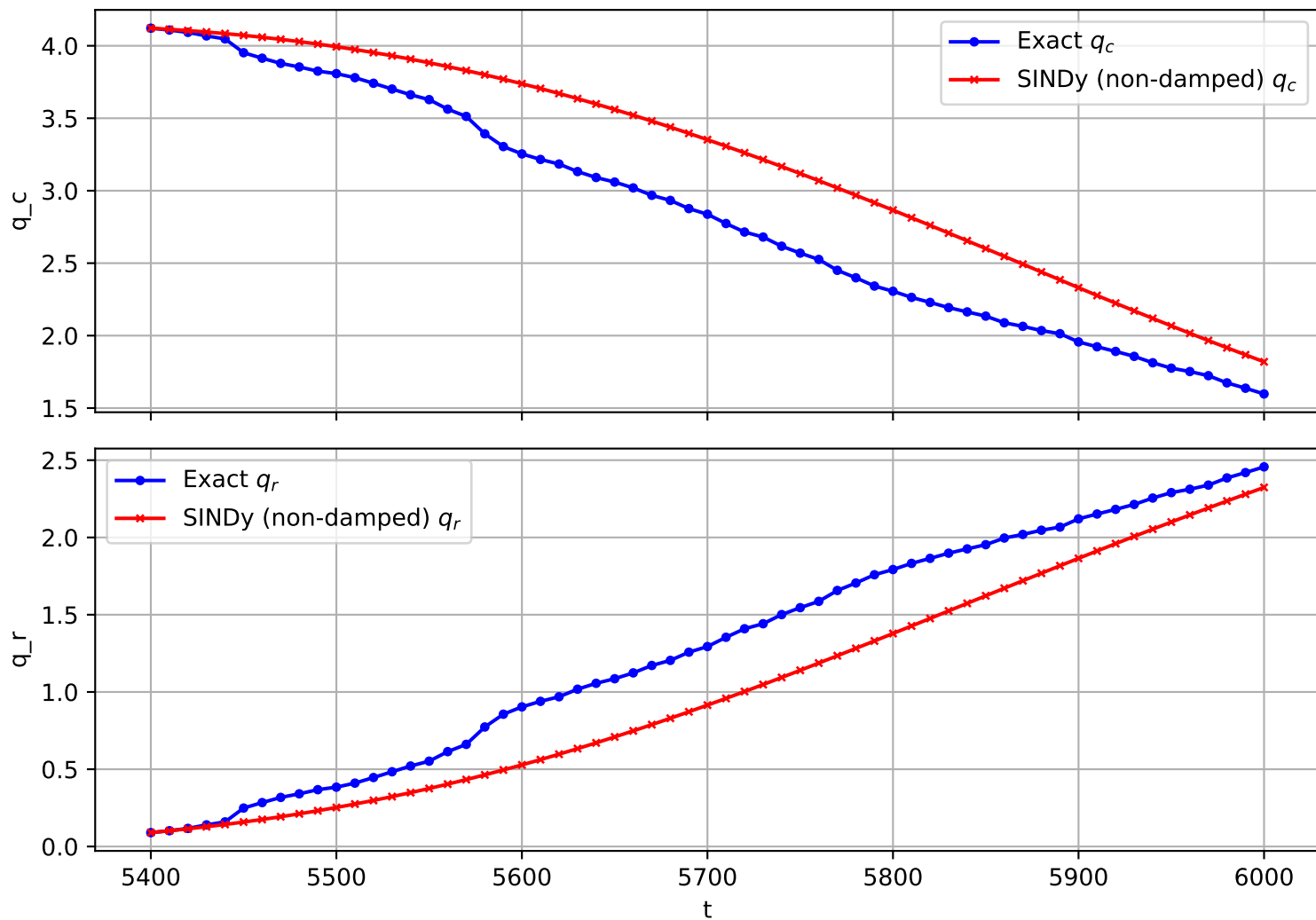
Trajectory 73 (non-damped)
