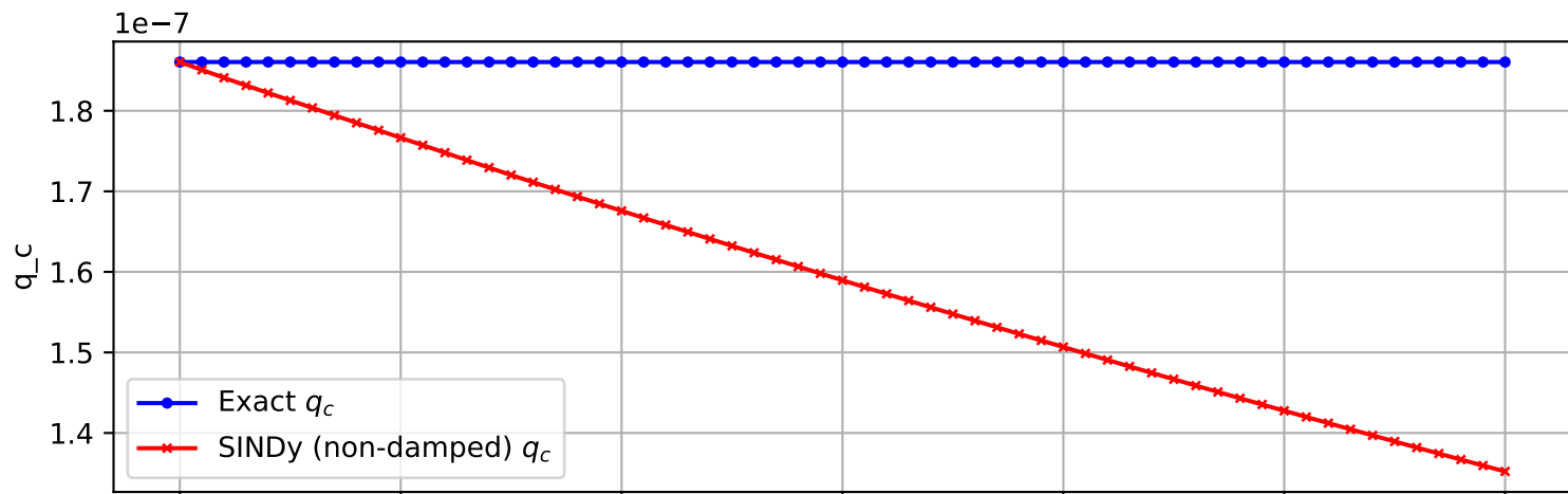
Trajectory 80 (non-damped)
