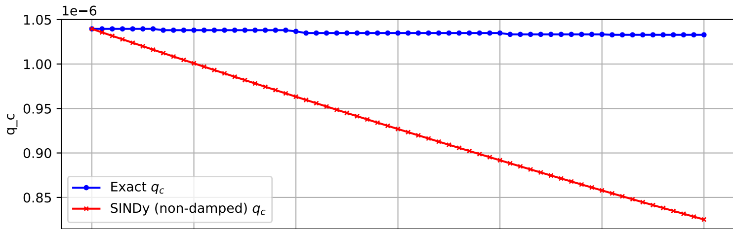
Trajectory 81 (non-damped)
