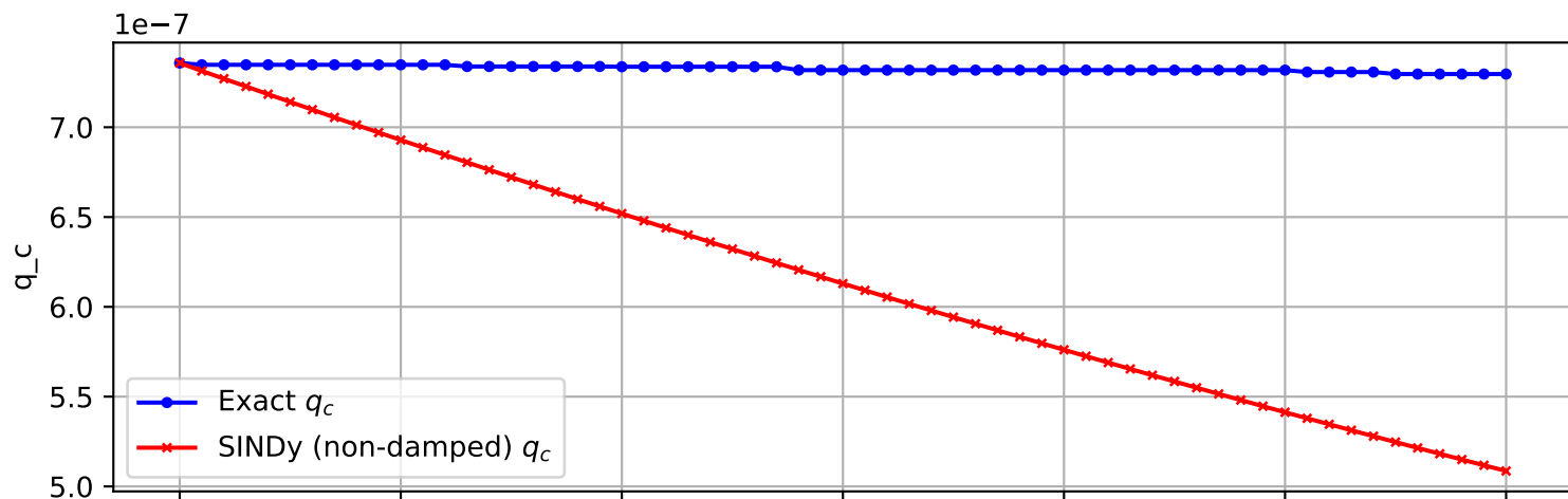
Trajectory 96 (non-damped)
