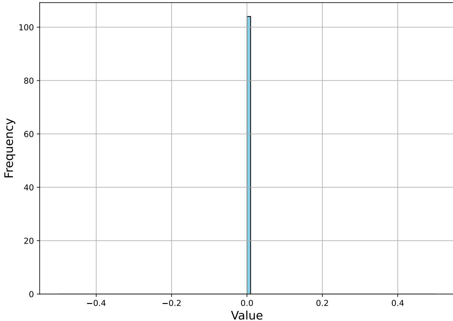
Variable 0, feature 2: x_0^2
