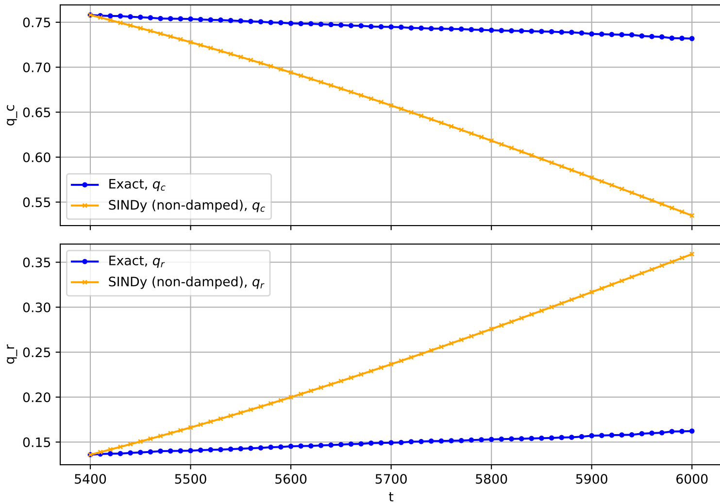
Trajectory No. 1013
