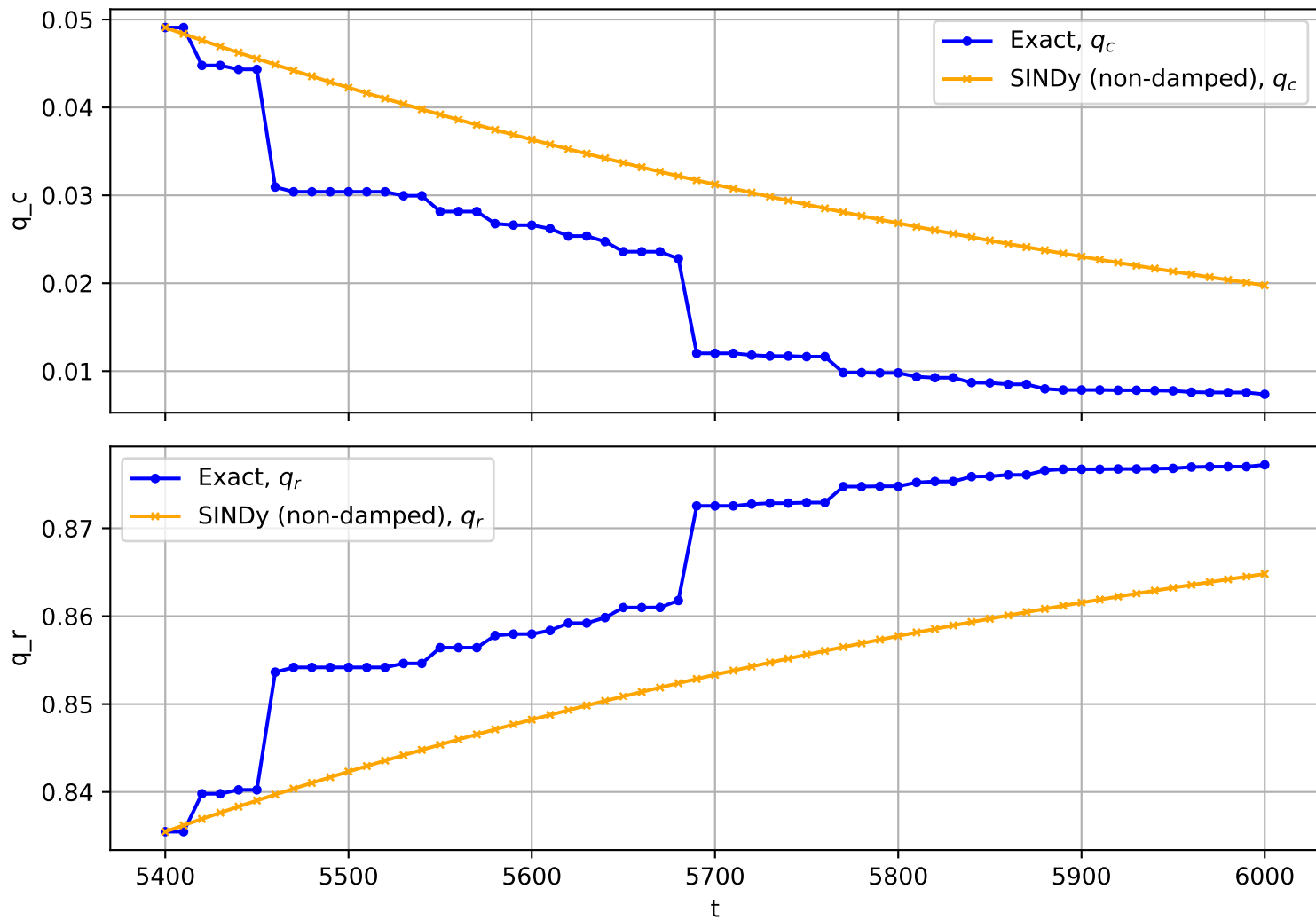
Trajectory No. 1017
