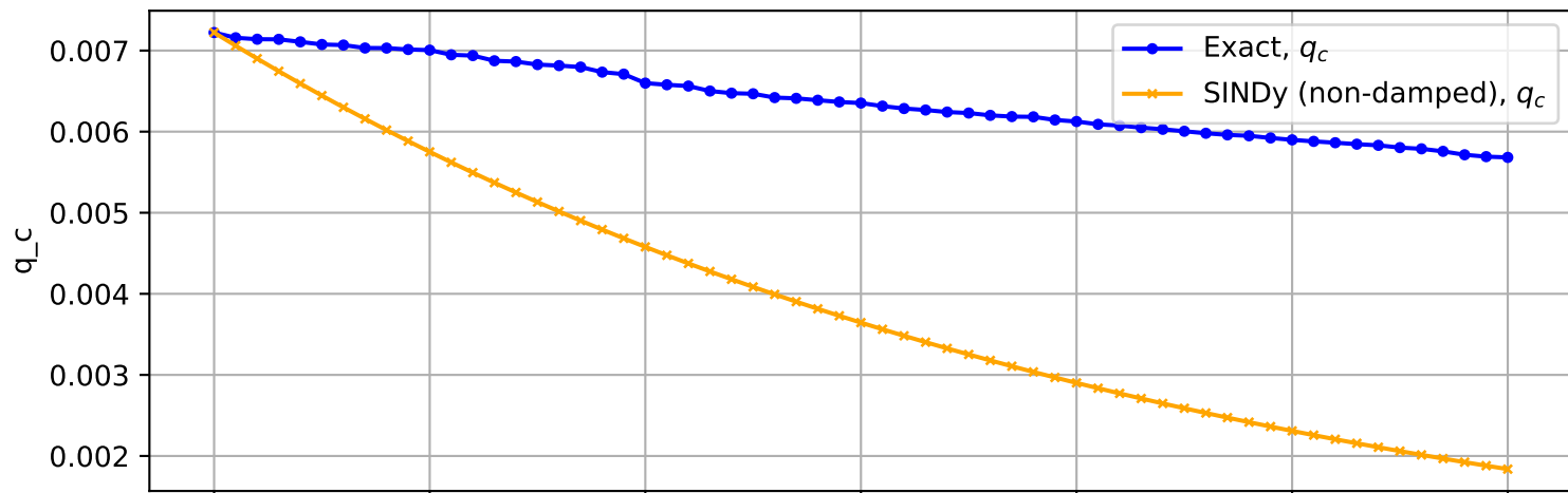
Trajectory No. 1047
