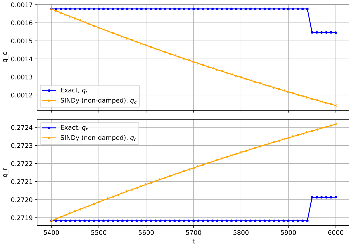
Trajectory No. 1119
