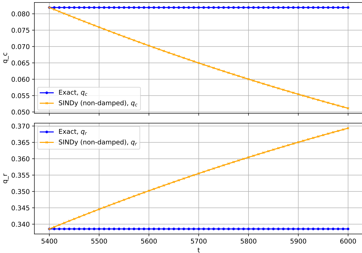
Trajectory No. 112
