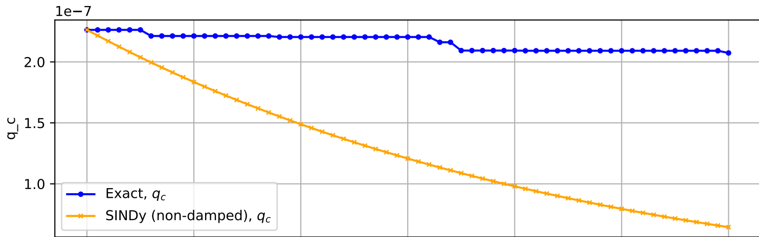
Trajectory No. 1171
