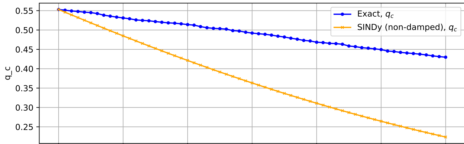
Trajectory No. 1189
