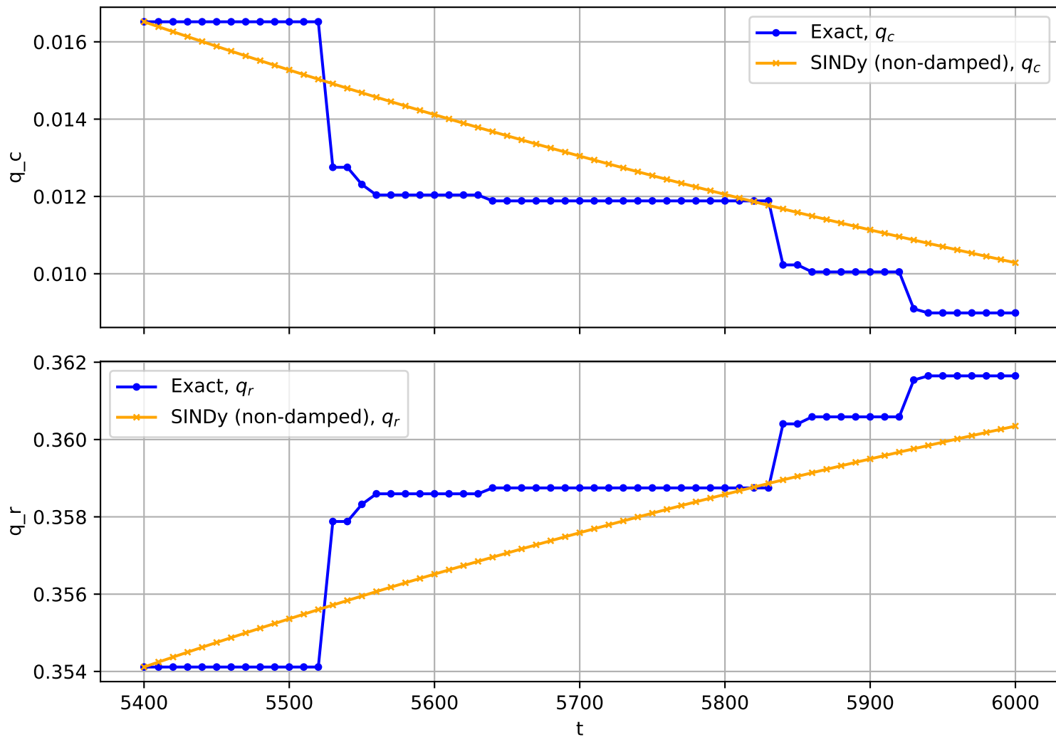
Trajectory No. 1236
