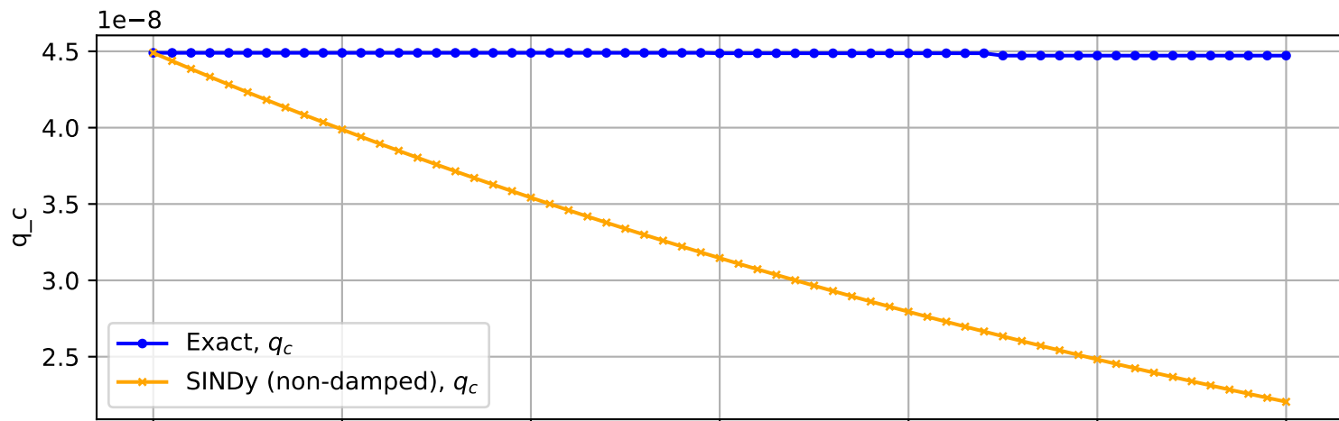
Trajectory No. 1241
