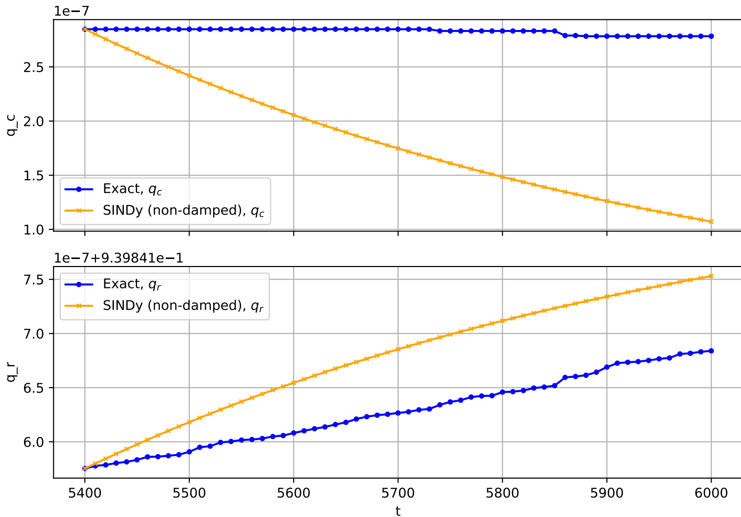
Trajectory No. 1244
