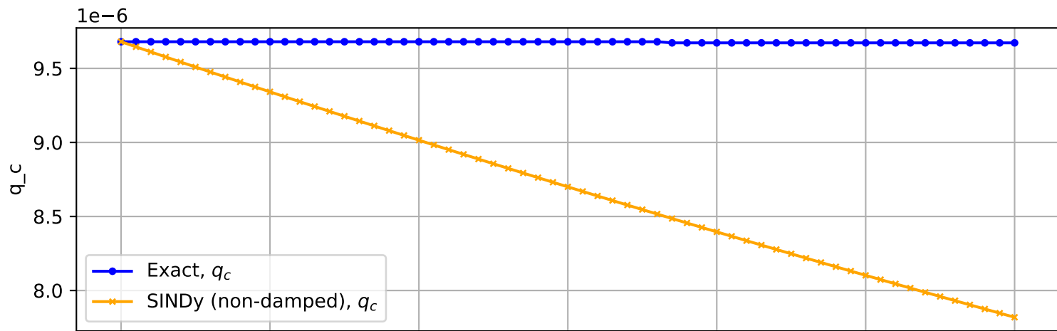
Trajectory No. 1278
