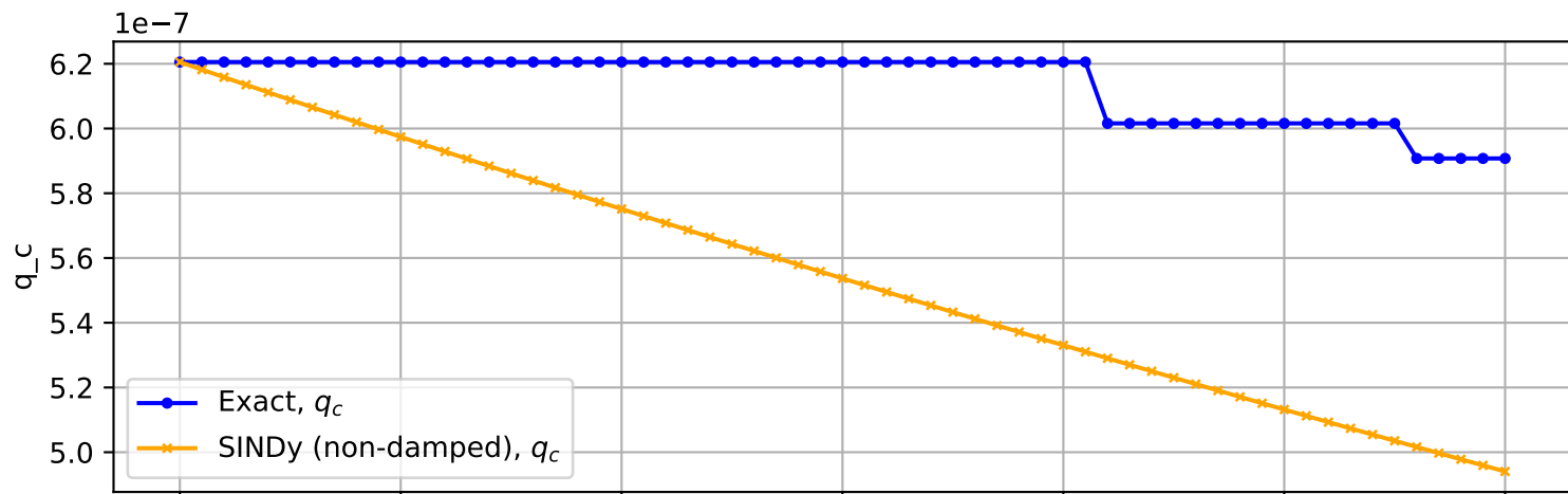
Trajectory No. 1280
