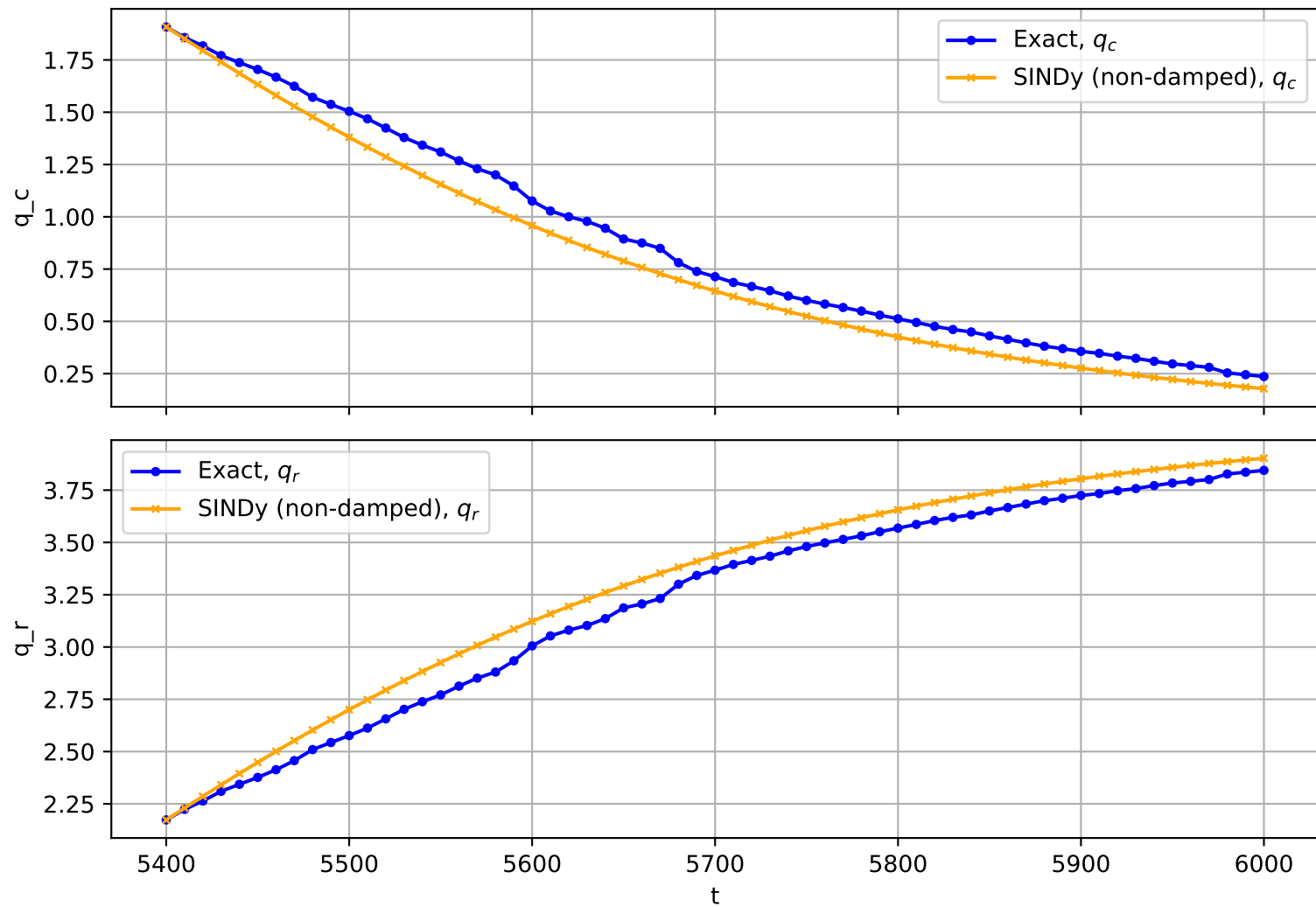
Trajectory No. 132
