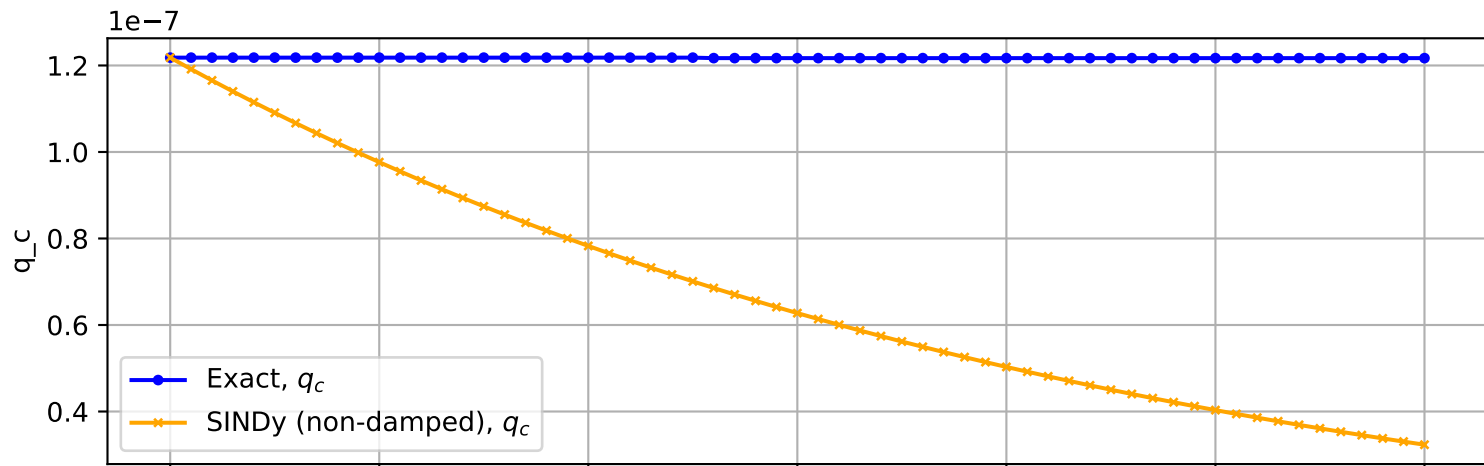
Trajectory No. 1320
