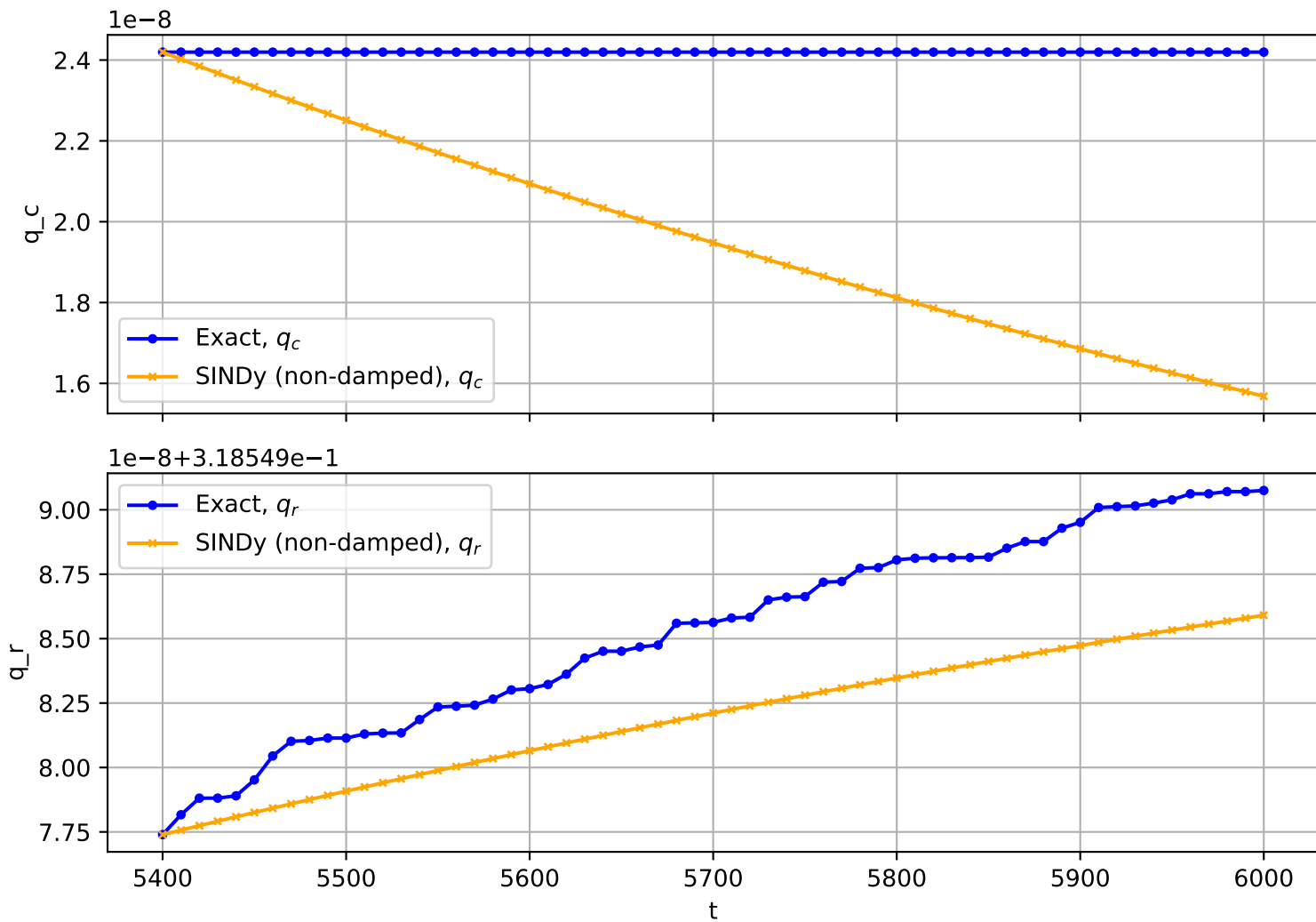
Trajectory No. 1336
