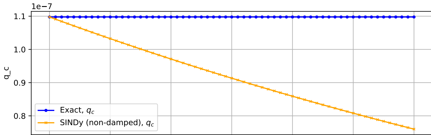
Trajectory No. 1344
