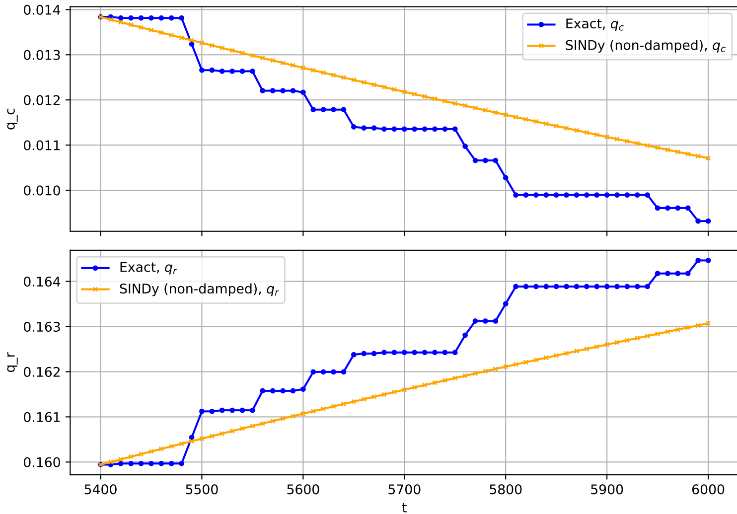
Trajectory No. 1352
