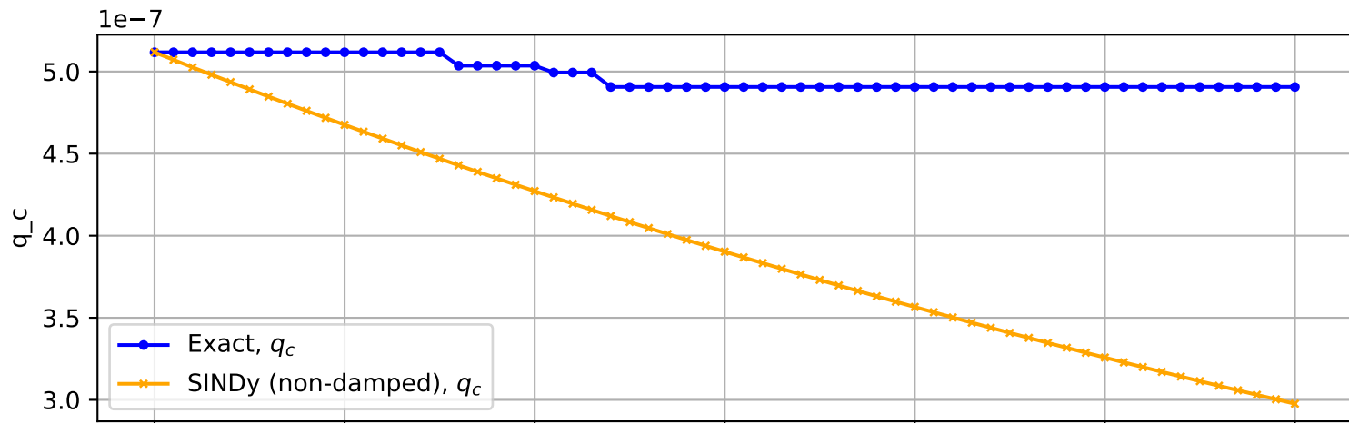
Trajectory No. 1363
