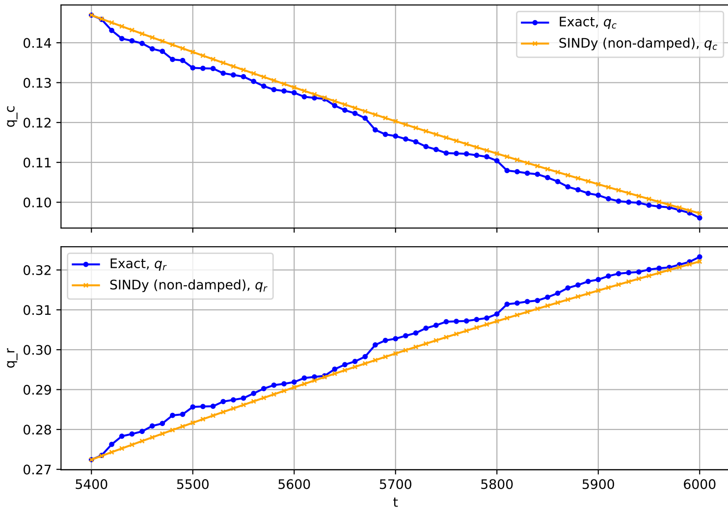
Trajectory No. 1392
