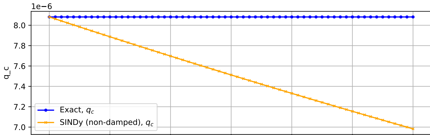
Trajectory No. 14
