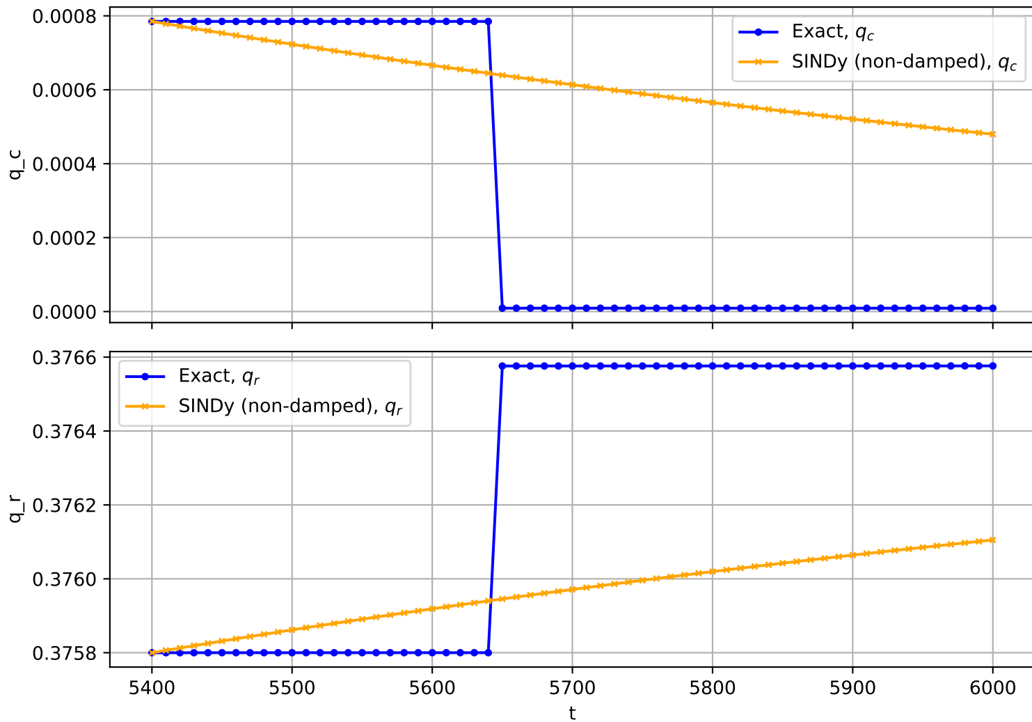
Trajectory No. 1416
