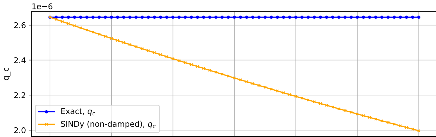
Trajectory No. 1440
