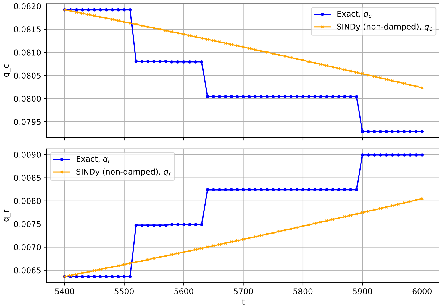
Trajectory No. 1444
