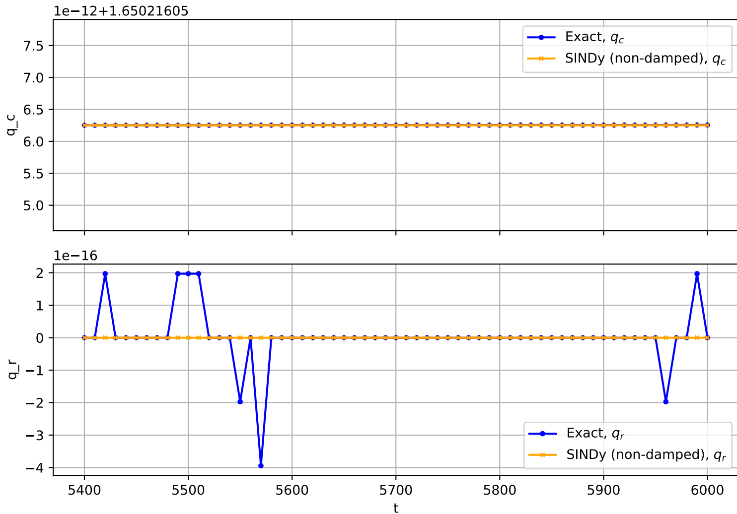
Trajectory No. 147
