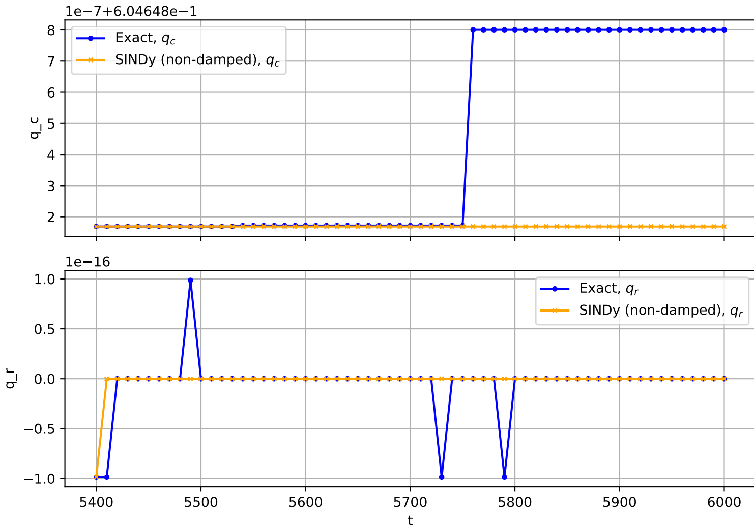
Trajectory No. 1525
