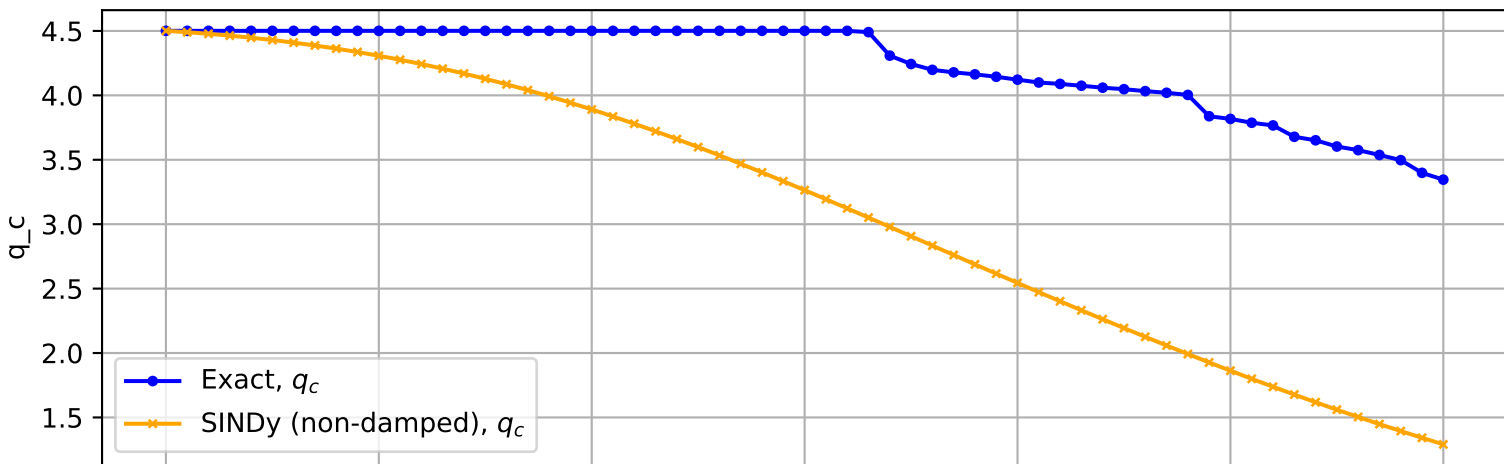
Trajectory No. 153
