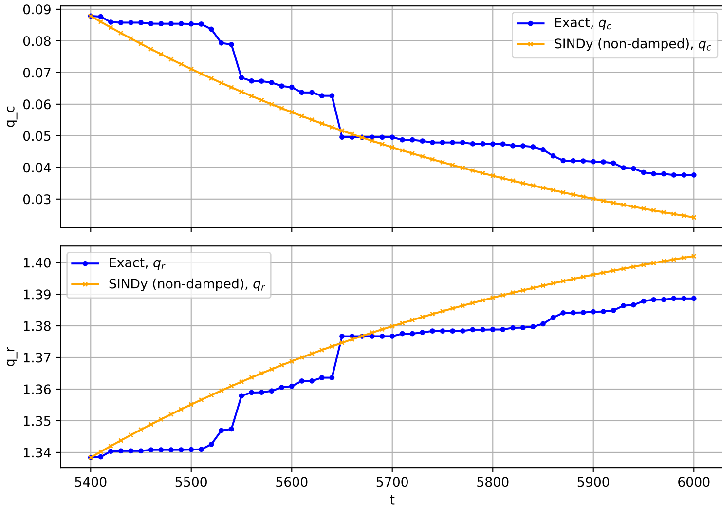
Trajectory No. 1544
