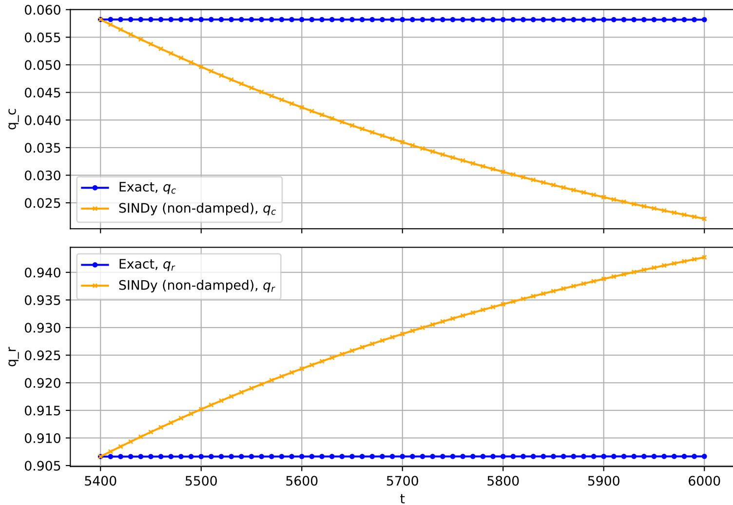
Trajectory No. 1564
